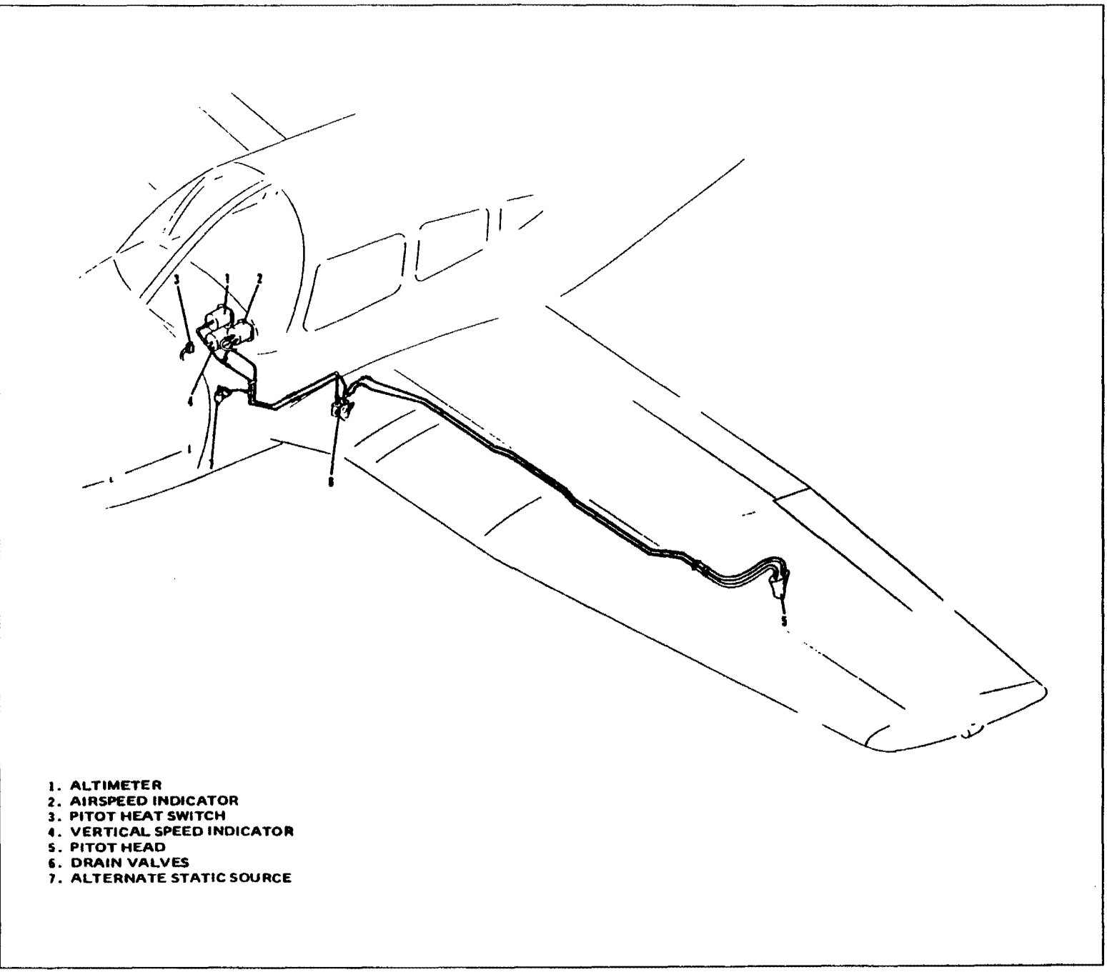
PITOT-STATIC SYSTEM
