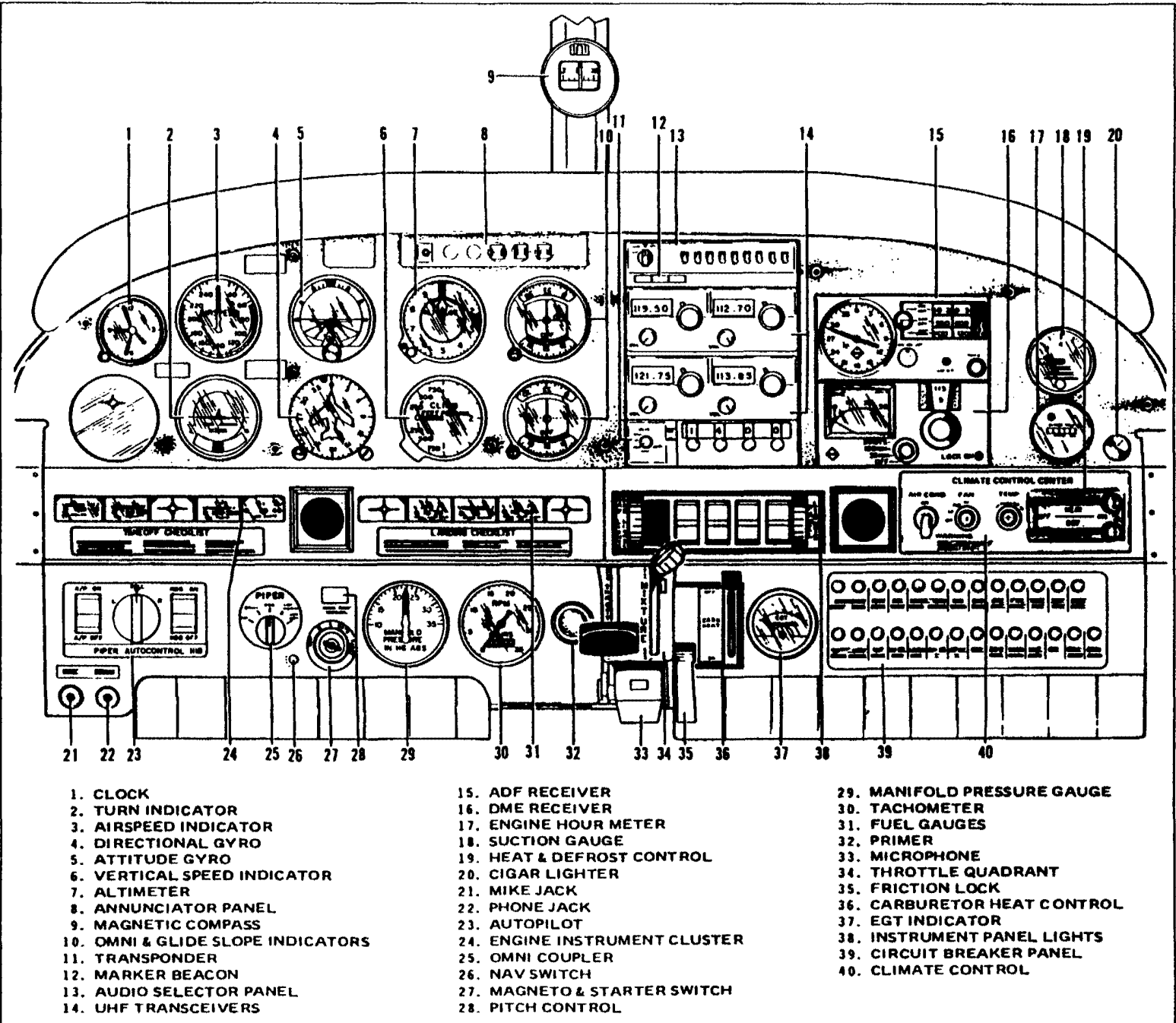
INSTRUMENT PANEL
