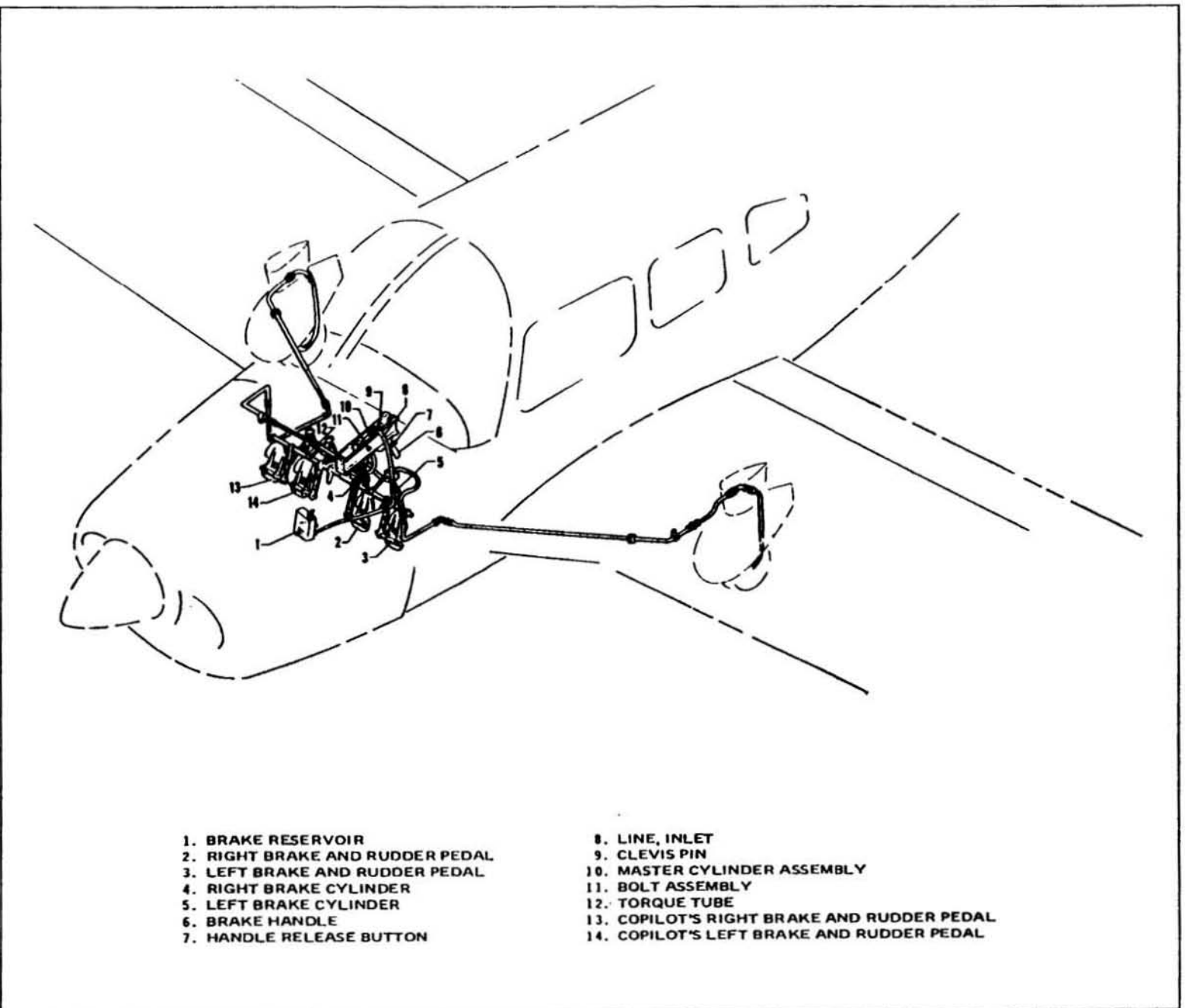
BRAKE SYSTEM
